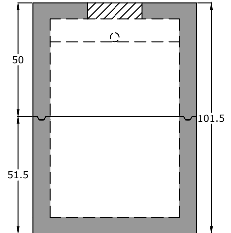
End View
