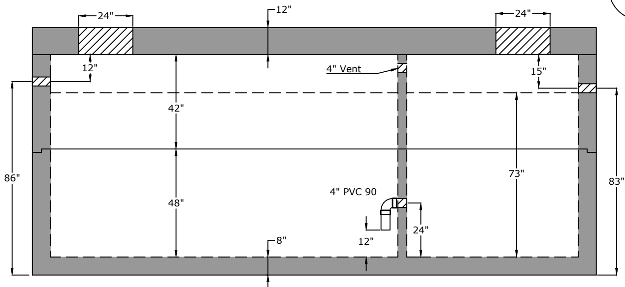
Side View
