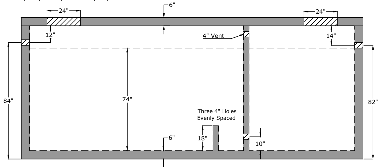
Side View
