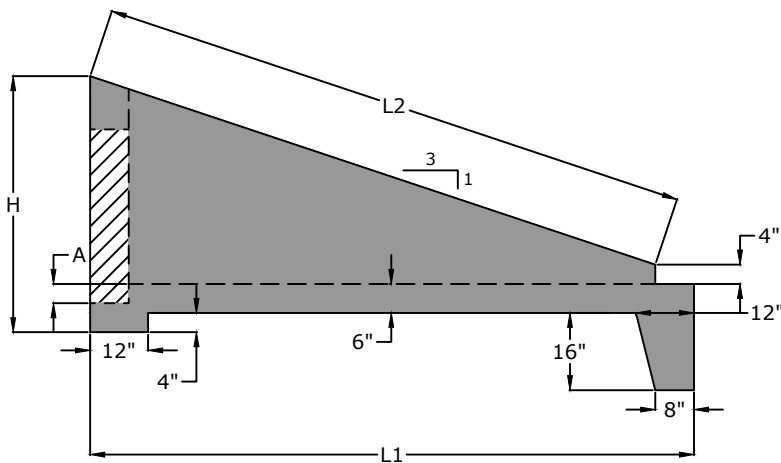
Dimensions (inches)
