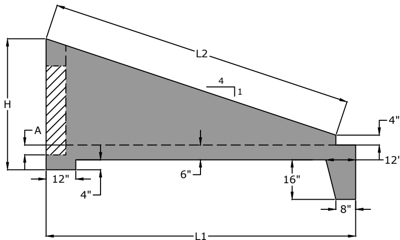
Dimensions (inches)
