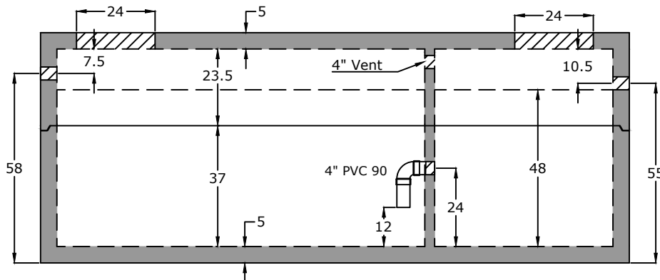
Side View
