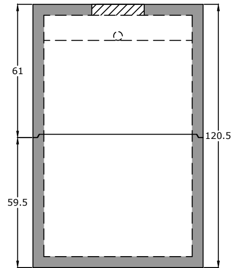
End View
