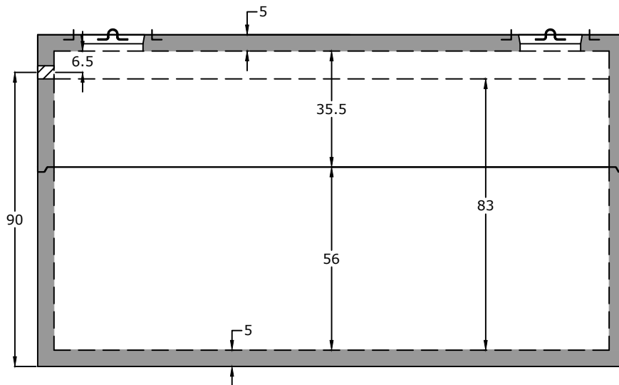
Side View
