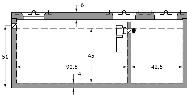
Side View
