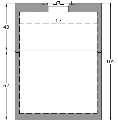
End View
