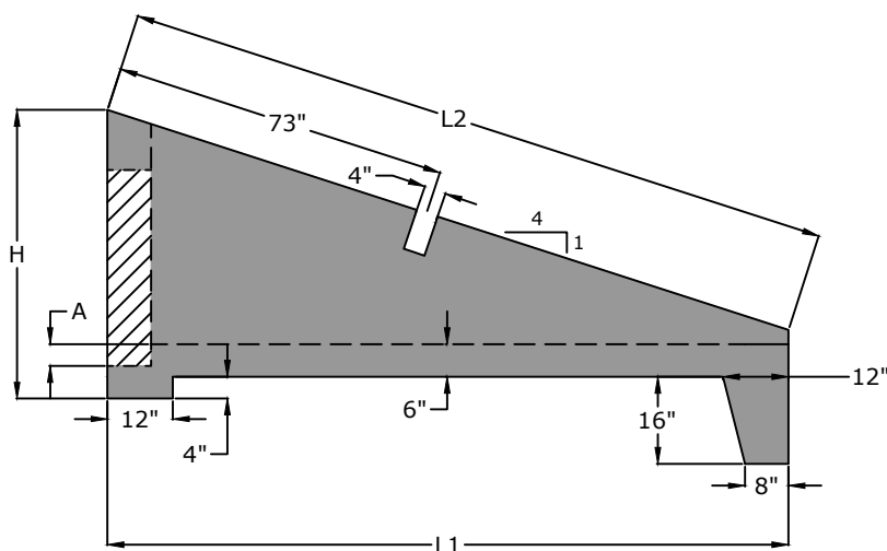
Dimensions (inches)
