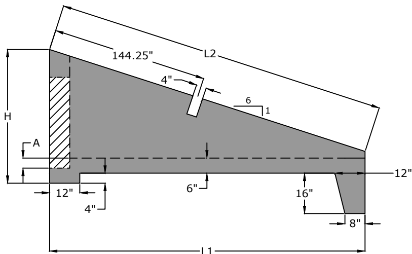
Dimensions (inches)
